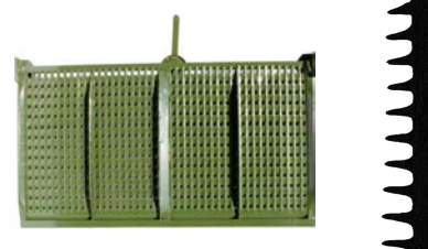
UCZ-12768 (AZ42291) EXTENSION SIEVE 1230X460 (1174)
